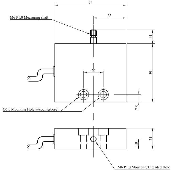
DPU-0.4 to DPU-110 Dimensions in mm
