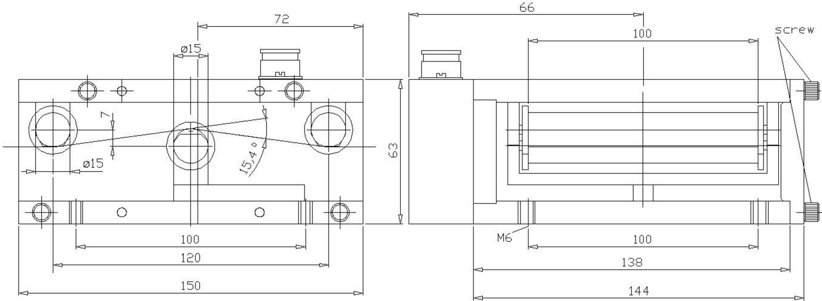
Dimensions of Online Sensor Model TSB2
