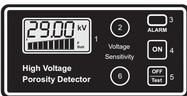
CONTROL LAYOUT
